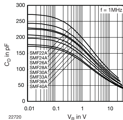
Fig. 6 - Typical Capacitance C D vs. Reverse Voltage V R
