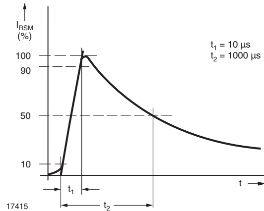
Fig. 4 - Pulse Waveform
